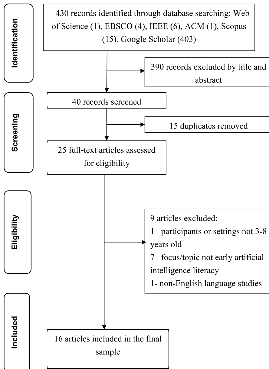
Fig. 1. PRISMA diagram of included articles in the scoping review.
